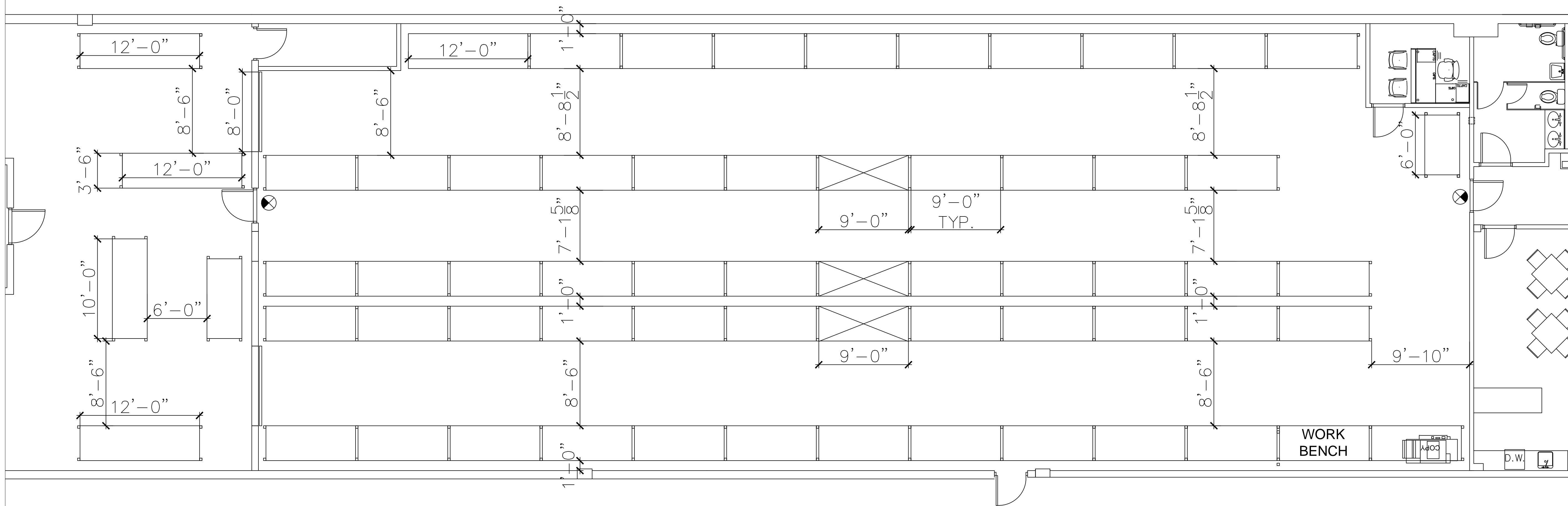
WAREHOUSE RACKING PLAN
